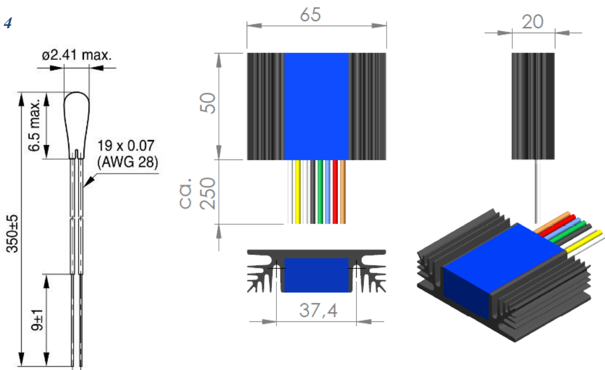
Sensor: QC-TE-BU-350
